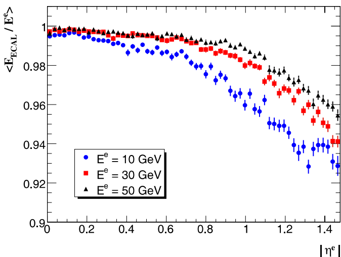
Fig. 10. The true energy reaching the ECAL barrel front face normalized to the initial energy as a function of the pseudorapidity \eta for electrons of 10, 30 and 50 GeV energy. To compute the true energy reaching the ECAL, only photons with energy greater than 10 MeV are considered
