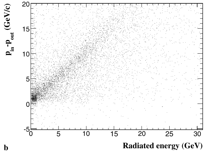
Fig. 9. Estimation of the bremsstrahlung radiated energy using the GSF track parameters, for electrons with p_T^e = 10 GeV/ c ; a track momentum evaluated at the vertex ( full histogram ) and at the outermost hit ( dashed-dotted histogram ); b difference between track momentum at vertex and at outermost state against the energy radiated via bremsstrahlung photons along the electron trajectory. The momentum is obtained from the weighted mean of the Gaussian mixture
