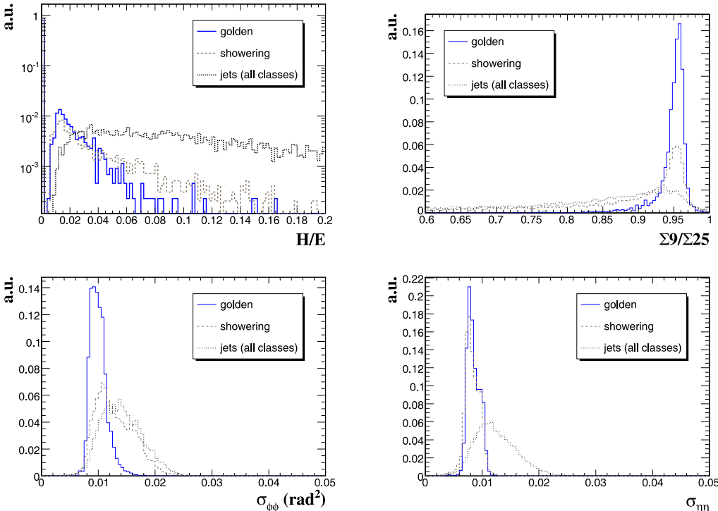
Fig. 21. Distributions of electron identification observables in the ECAL barrel. The distributions of shower shape observables are shown for different classes of electrons, and in comparisons with distributions for “fake” electron candidates from QCD jet background. Similar distributions with larger spread are observed for electrons in the endcaps
