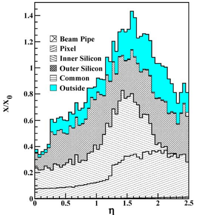
Fig. 1. Material budget [9] in front of the ECAL in units of radiation length
