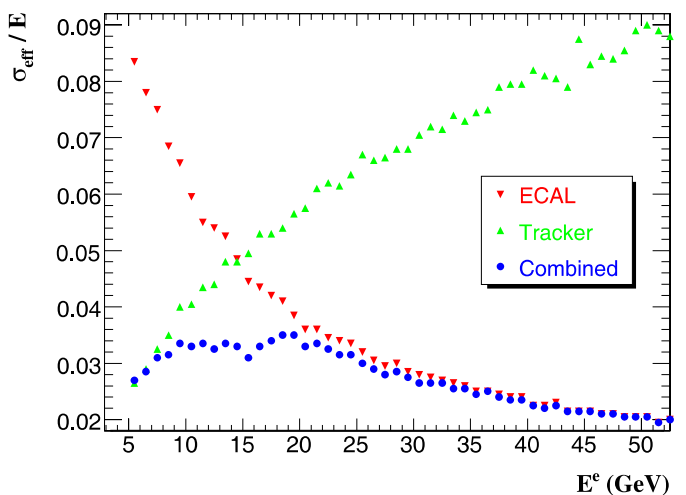
Fig. 17. The resolutions as measured by the relative effective RMS of the corrected supercluster energy ( downward triangles ), the reconstructed track momentum at origin ( upward triangles ), and of the combined electron momentum estimate ( circles ) as a function of the electron incident energy for electrons in the ECAL barrel
