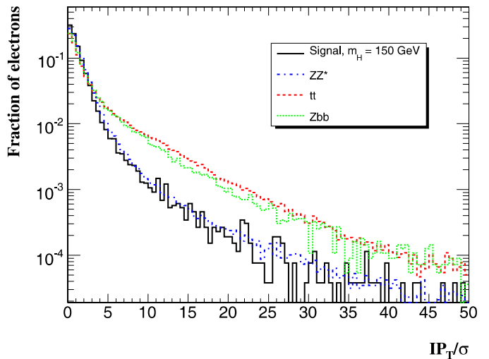
Fig. 19. The distributions of the normalized transverse impact parameter \text{IP}_{\text{T}}/\sigma_{\text{IP}_{\text{T}}} for pre-selected electrons from the SM Higgs boson decaying in H \rightarrow ZZ^* \rightarrow e^+e^-e^+e^- ( m_H = 150 \text{ GeV}/c^2 ) and for pre-selected electrons from the ZZ^* , t\bar{t} and Zb\bar{b} backgrounds
