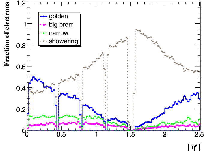
Fig. 11. The fraction of electron population in the different classes as a function of the generated pseudorapidity for initial energies between 5 and 100 GeV
