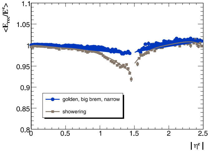
Fig. 14. Mean of the reconstructed supercluster energy E_{\text{rec}} after f(N_{\text{cry}}) correction divided by the generator electron energy E^e for different classes and as a function of the pseudorapidity. In the \eta range of the ECAL endcaps, E^e is taken as the generated initial energy minus the energy measured in the preshower detector
