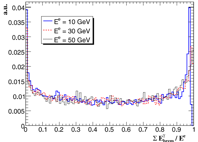
Fig. 2. Distribution of the fraction, \sum E_{brem}^\gamma / E^e , of the generated electron energy ( E^e ) radiated as bremsstrahlung photons ( \sum E_{brem}^\gamma ) for electrons of 10, 30 and 50 GeV. The true emission of bremsstrahlung photons has been integrated up to a radius corresponding to the ECAL inner radius
