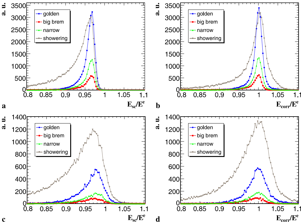
Fig. 12. The distribution of the raw and fully corrected reconstructed electron energy normalized to the generated energy, for the different electron classes. Distributions obtained for uniformly distributed electrons of energies between 5 and 100 GeV are shown separately for the \eta range of the a, b barrel and c, d endcaps. The distributions are obtained a, c before ( E_{\text{sc}} ) and b, d after ( E_{\text{corr}} ) application of all energy scale corrections (as explained in the text). For the endcaps, E_{\text{sc}} and E_{\text{corr}} includes the energy deposited in the preshower
