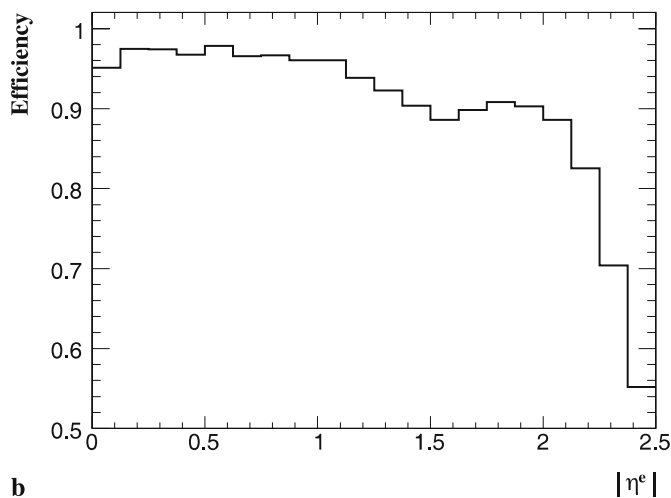
Fig. 4. Electron track reconstruction efficiency a as a function of p_T and b as a function of |\eta| , for electrons uniformly distributed in p_T between 5 and 50 GeV/c. In a , the efficiency is shown averaged over the full ECAL barrel and endcaps \eta range ( full line ) and for the barrel only ( dotted line )
