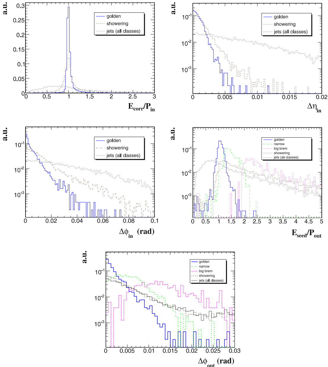
Fig. 22. Distributions of electron identification observables in the \eta range of the ECAL barrel. The distributions of track-cluster matching observables are shown for different classes of electrons, and in comparisons with distributions for “fake” electron candidates from QCD jet background. Similar distributions with larger spread are obtained for electrons in the endcaps
