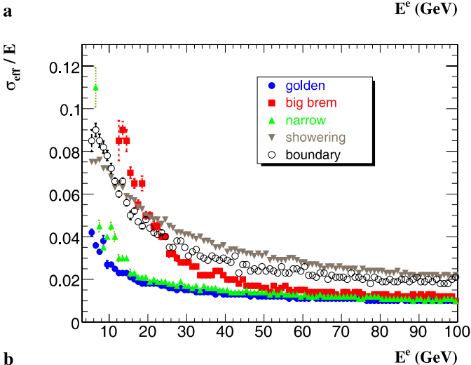
Fig. 16. The energy measurement precision as a function of the generated electron energy for the different classes and for electrons in the barrel: a resolution as obtained from a fit of the Gaussian part of the corrected energy distribution; b resolution as obtained computing the half width of the smallest window that contains 68.3% of the distribution. The line corresponds to a fit for the golden electrons using a standard calorimeter resolution function, as described in the text
