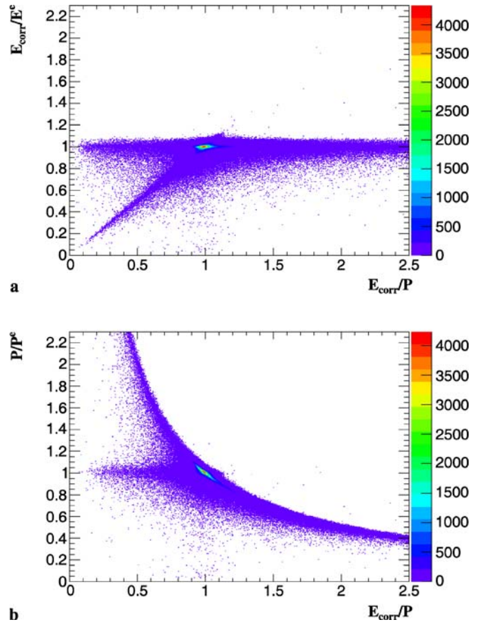
Fig. 15. The momentum estimate from the ECAL and the tracker as a function of E/p for electrons in the ECAL barrel: a corrected supercluster energy E_{\text{corr}} normalized to the initial electron energy as a function of E_{\text{corr}}/p ; b reconstructed track momentum at origin p normalized to the initial electron energy as a function of E_{\text{corr}}/p
