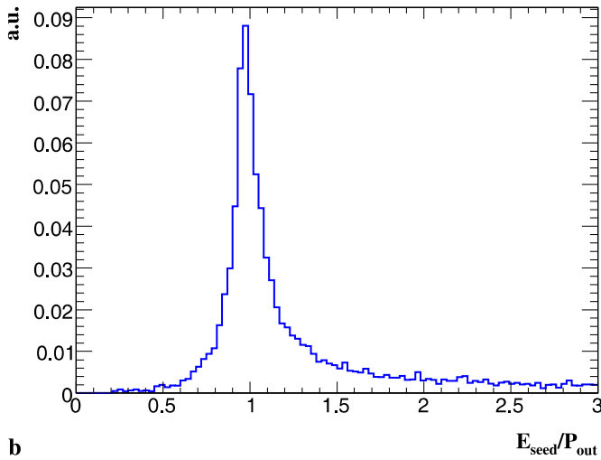
Fig. 8. Distributions of E/p for p_T^e = 10 GeV/ c electrons; a supercluster energy over track momentum measured at vertex; b supercluster seed energy over track momentum estimated at the last hit
