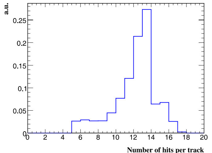
Fig. 5. Number of reconstructed hits per track for electrons of p_T^e = 10 GeV/c
