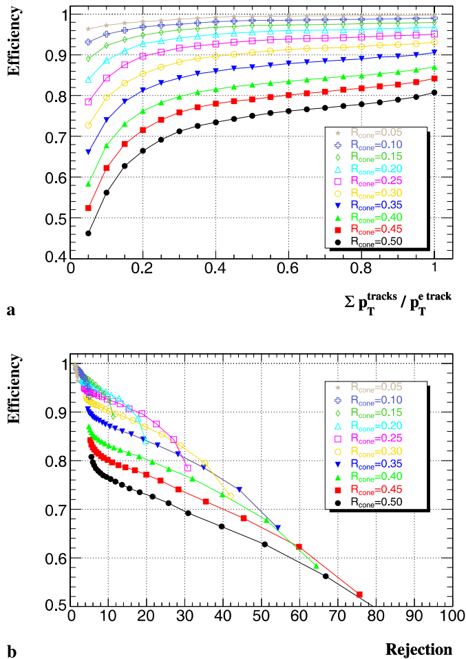
Fig. 20. Performance of track isolation in the channel H \rightarrow ZZ^* \rightarrow e^+e^-e^+e^- after the pre-selection described in the text: a efficiency on the Higgs boson signal as a function of the isolation variable and for different cone sizes; b efficiency for the Higgs boson signal as a function of the rejection obtained against the t\bar{t} background
