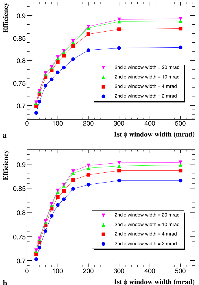
Fig. 3. Efficiency of the pixel matching for electron tracks reconstruction as a function of the \phi window for the finding of the first pixel: a p_T^e = 7 GeV/ c electrons and b p_T^e = 10 GeV/ c electrons. Plots are shown for varying the setting of the \phi window, in which a second pixel hit is searched for
