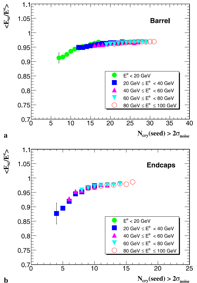
Fig. 13. Mean of the raw reconstructed supercluster energy E_{\text{sc}} divided by the generator electron energy E^e as a function of the number of crystals in the seed cluster that contain an energy greater than 2\sigma_{\text{noise}} : a electrons in the ECAL barrel; b electrons in the ECAL endcaps. In the \eta range of the ECAL endcaps, E^e is taken as the generated initial energy minus the energy measured in the preshower detector. Only electrons with p_T > 5 \text{ GeV}/c and with no identified bremsstrahlung cluster are considered
