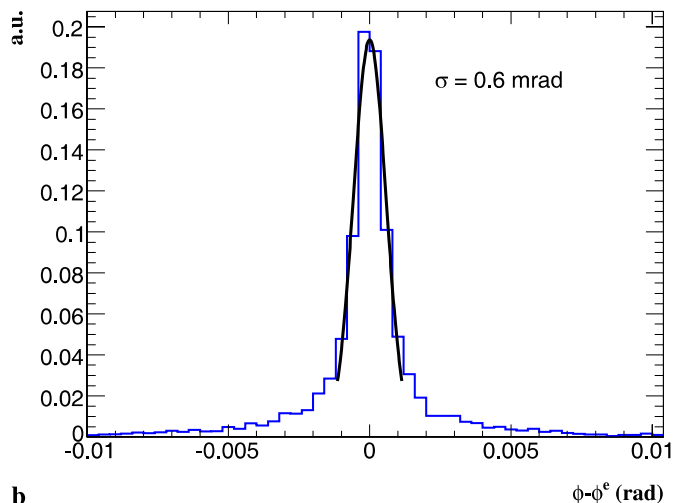
Fig. 7. Difference between the reconstructed track direction at vertex and the generated one: a \eta direction and b \phi direction for p_T^e = 10 GeV/ c electrons
