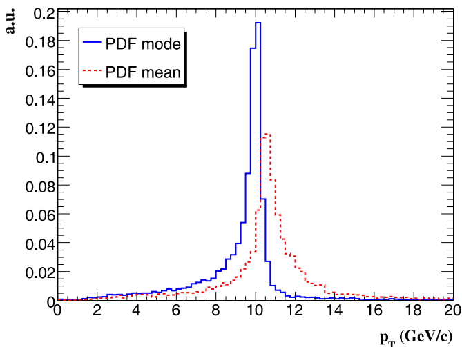
Fig. 6. Reconstructed p_T distribution for fixed p_T^e = 10 GeV/ c electrons, using the most probable value of the Gaussian mixture ( full histogram ) and using the weighted mean of the Gaussian mixture ( dashed histogram ) to evaluate the track momentum
